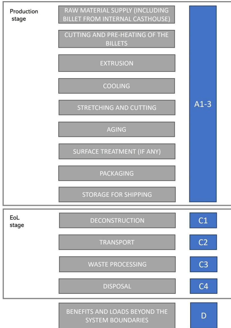
Figure 1. Scheme of the profiles manufacturing process occurring at Delhi
