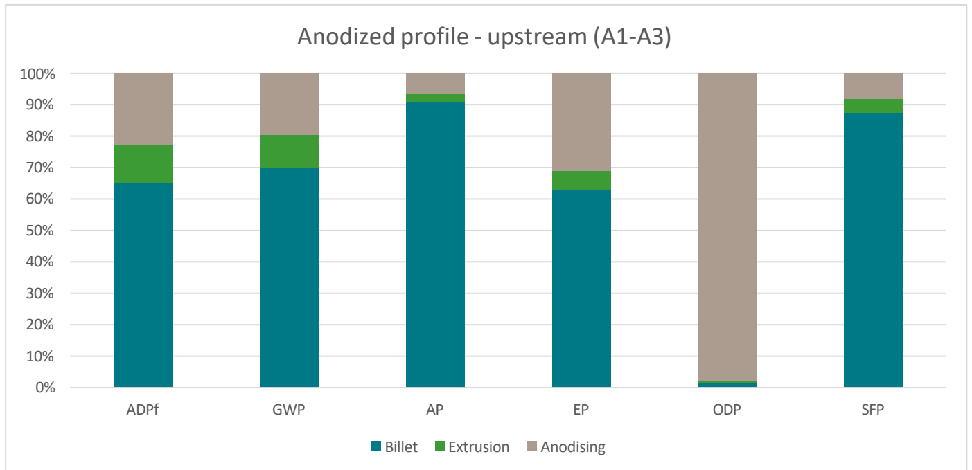
Figure 3. Relative contribution to upstream process of anodized profile
